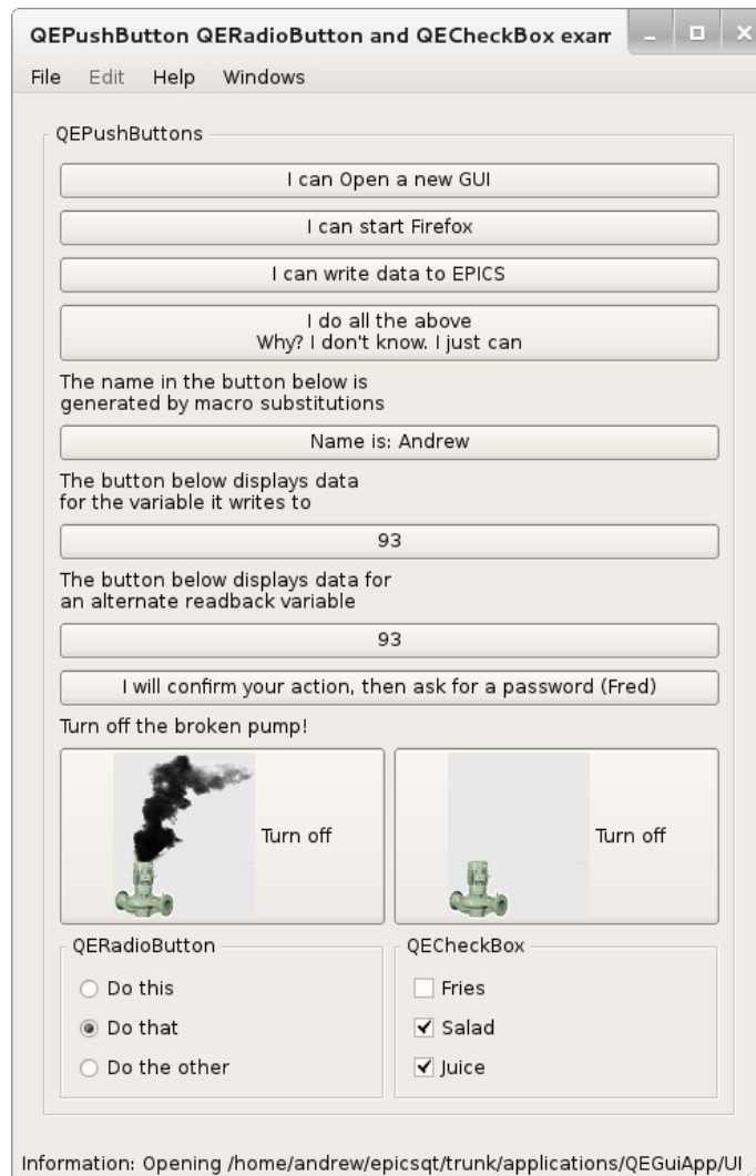
Figure 28 QEPushButton, QERadioButton and QECheckBox examples
