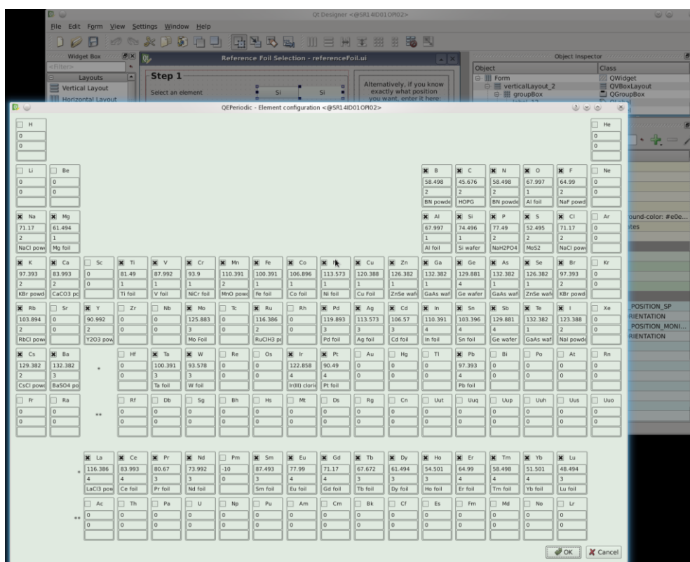
Figure 26 Editing the QEperiodic userInfo property - the relationship between each element and variable values
