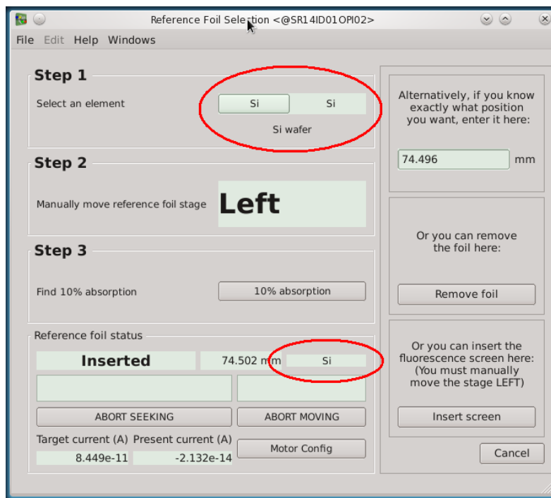
Figure 23 QEPeriodic used for both read-back and control by element.
