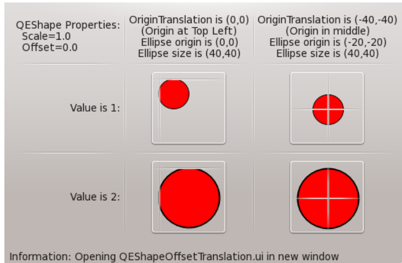
Figure 37 QEShape originTranslation example
