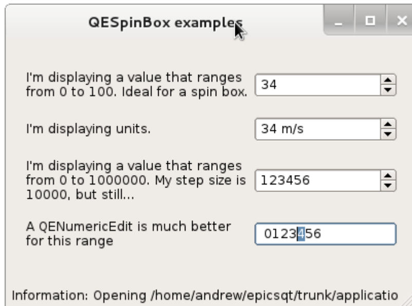
Figure 40 QESpinBox examples with a QNumericEdit where more appropriate
