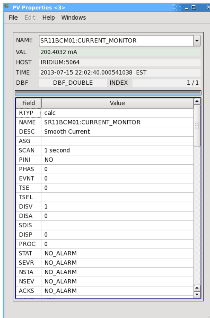
Figure 30 QEPvProperties widget example examining a calc record.
