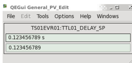
Figure 11 QEGeneralEdit example for a numeric for PV
