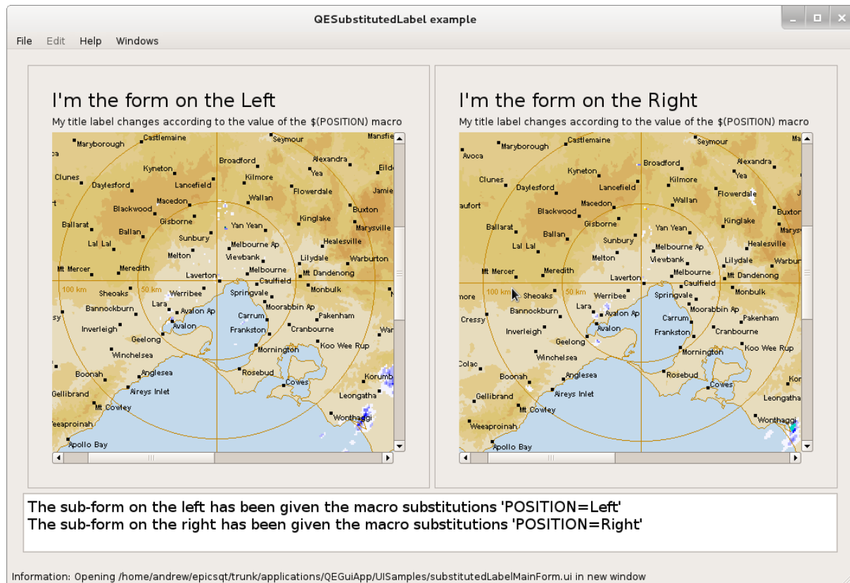
Figure 41 QESubstitutedLabel used to vary title in sub forms
