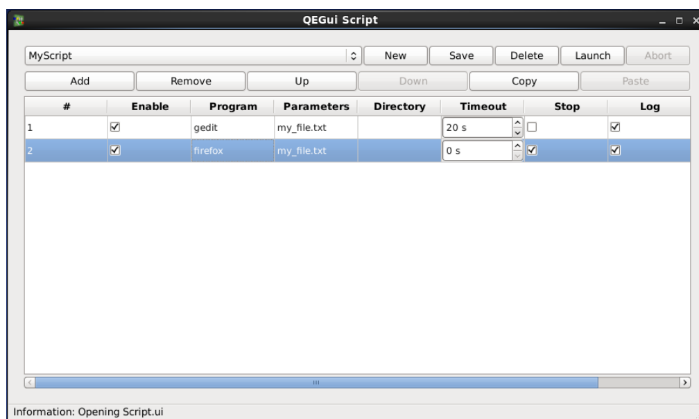
Figure 34 QEScript displaying a sequence of external programs to be executed(in this case "gedit" and "firefox")
