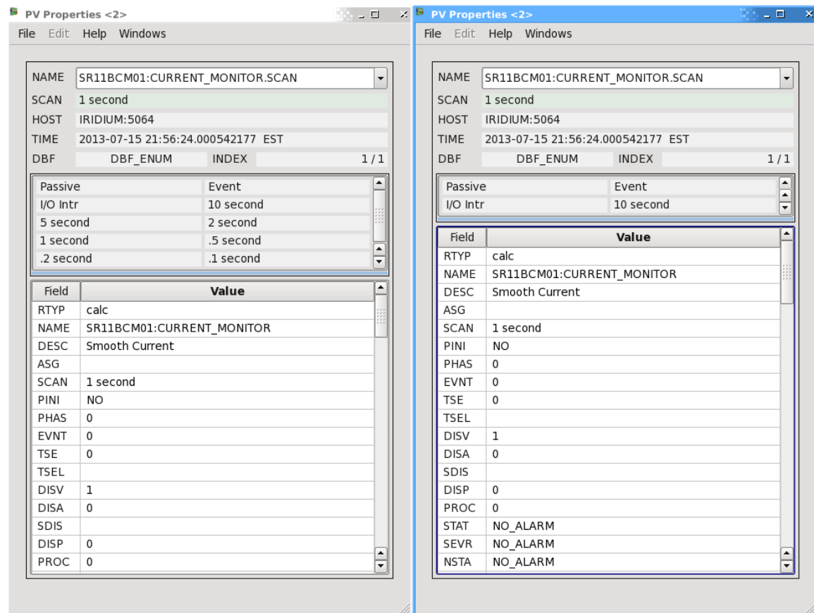
Figure 31 QEPvProperties widget example examining an enumeration PV.
