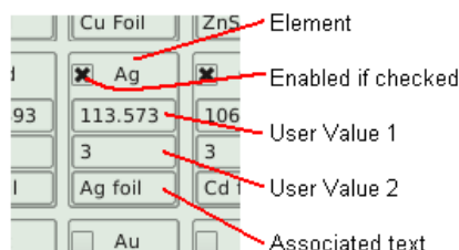
Figure 27 Editing the QEperiodic userInfo property - what is associated with each element
