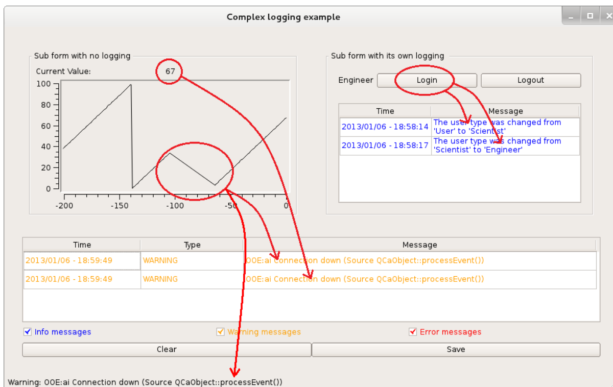
Figure 9 Complex logging example
